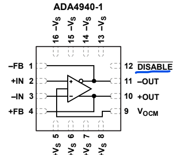
Figure 1. ADA4940-1
