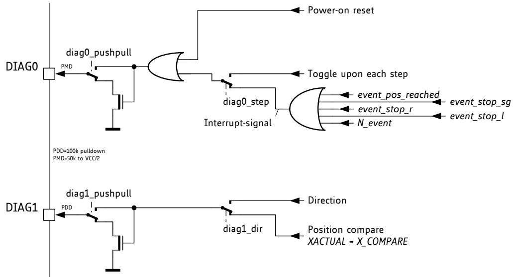
Figure 18.2 DIAG outputs with \text{SD\_MODE}=0
